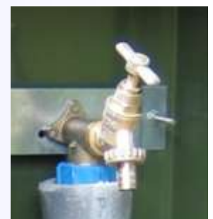
Hose Union Bib-tap 1/2" or 3/4" BS1010 DZR tap fitted Insulated MDPE pipe-work pre-installed
